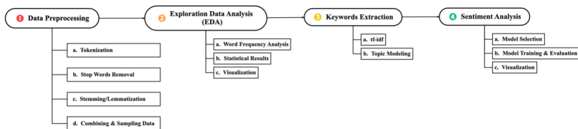
Figure 1. The Flow Chart of Text Mining Project
